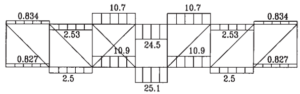
(c) SHEAR (KIPS)
