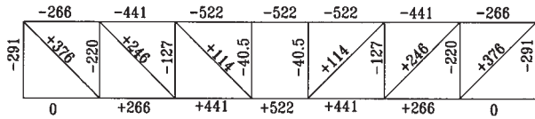
(a) AXIAL FORCE (KIPS) NOTE: TENSION IS POSITIVE
