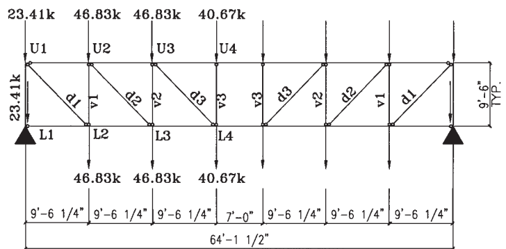
Fig. 3.1 Analysis of truss T1B—gravity loads.
